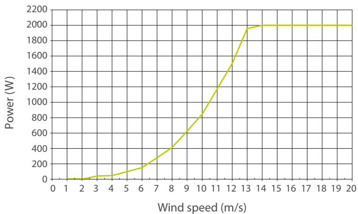
Power curve
